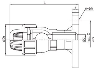
FLANGED END
